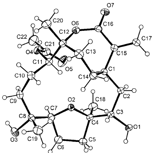
Figure 4. Molecular structure of 2 based on X-ray analysis.
